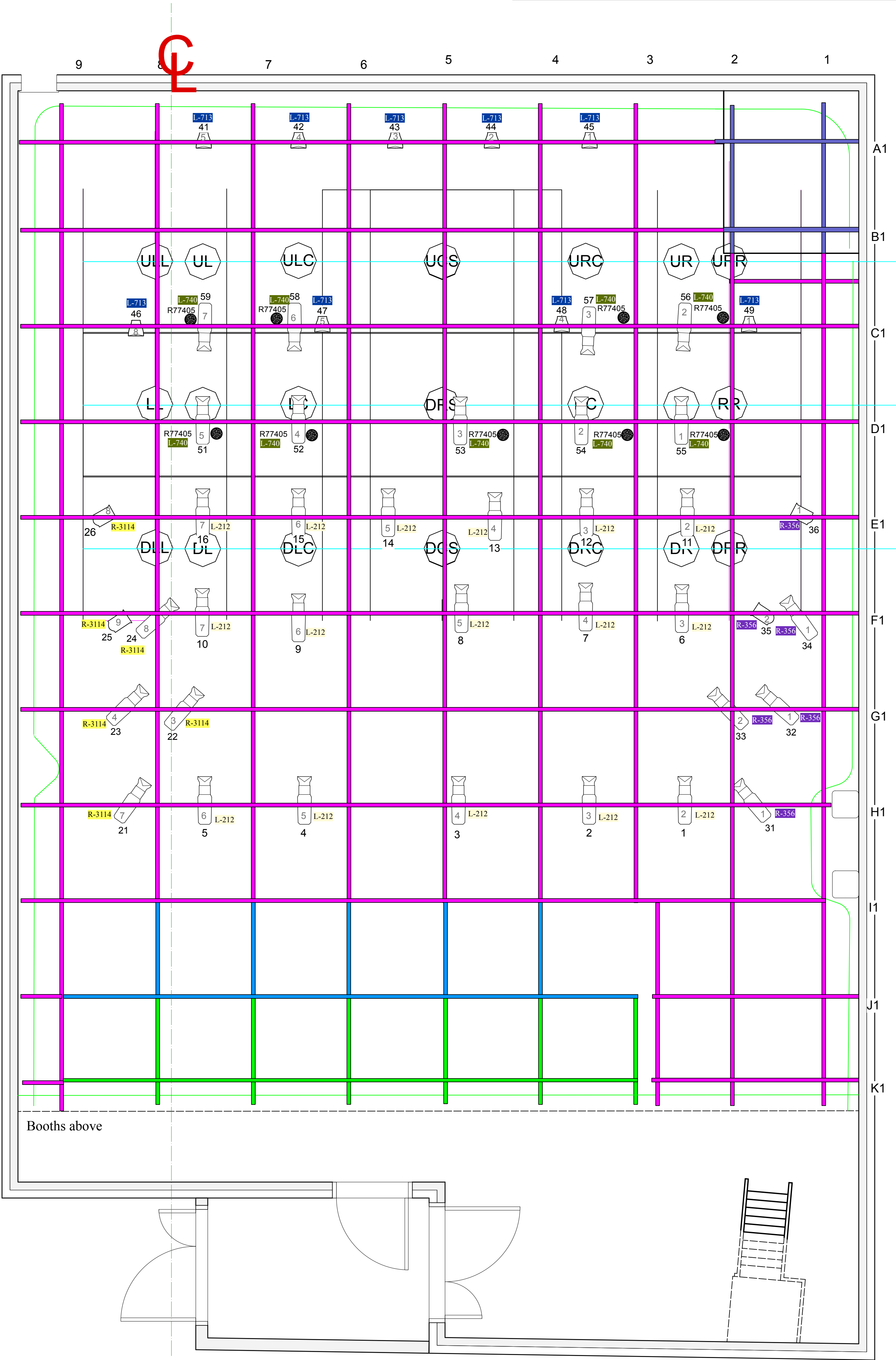
1 Lighting Plot Scale: 1:32
