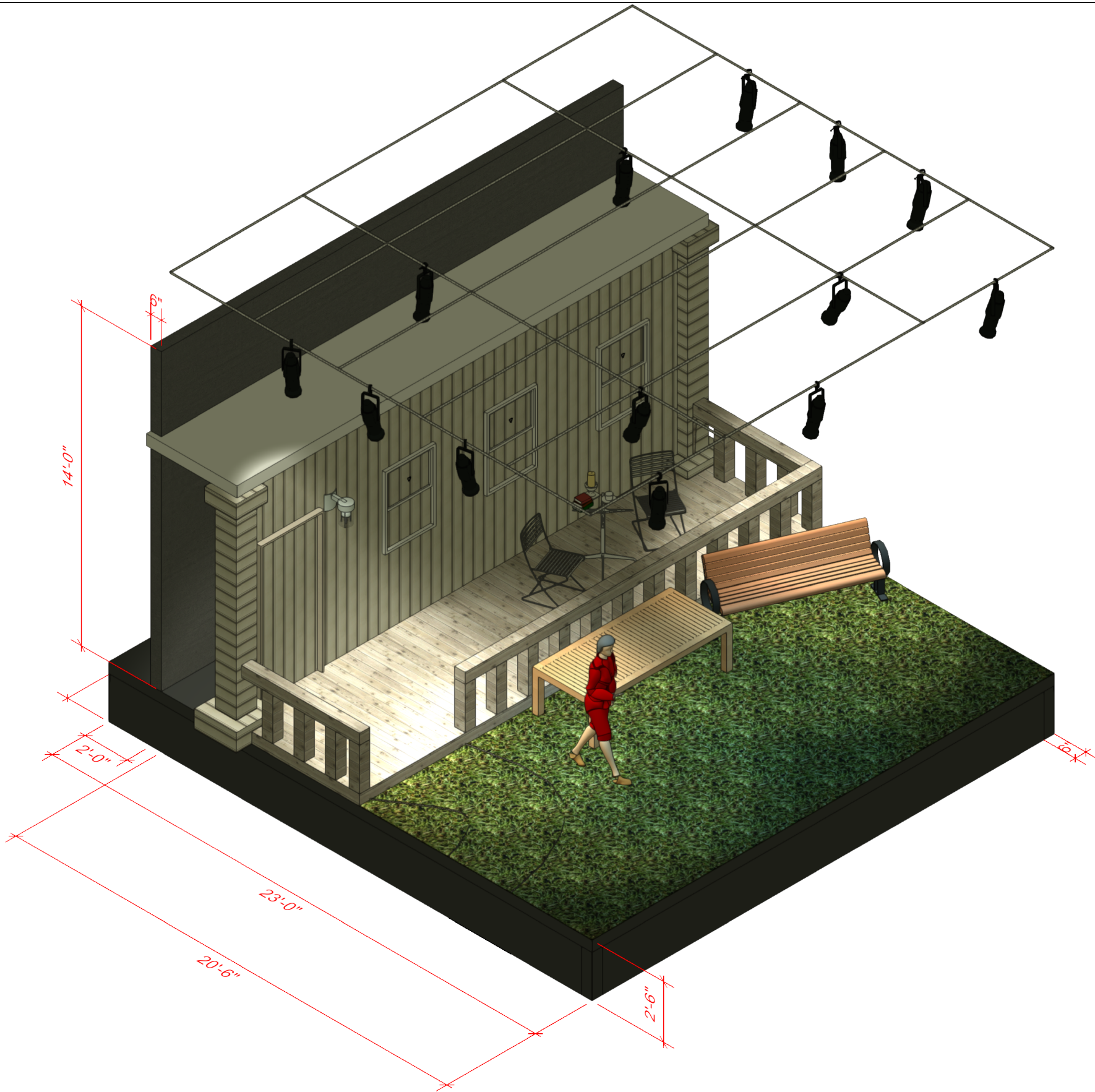
1 All My Sons - Light Motif 4 Scale: 1/4" = 1'-0"
